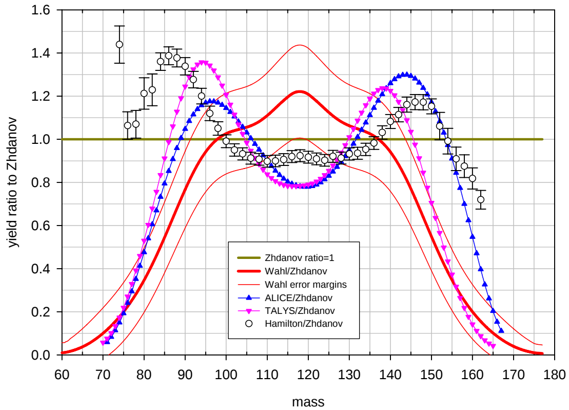
Benchmark A: ^{238}\text{U} 60 MeV proton induced fission, pre neutron emission yield ratio to Zhdanov
